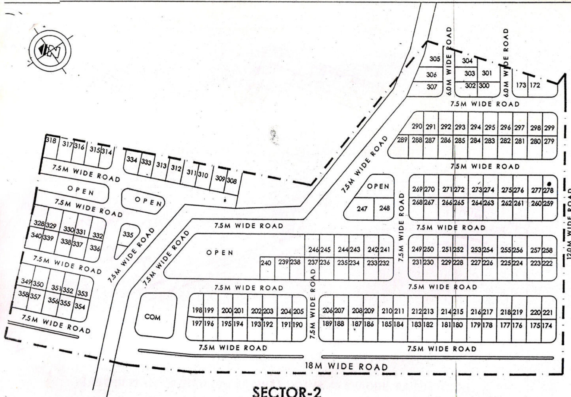
LAYOUT PLAN OF DEEN DAYAL AWAS YOJNA AT SHADDU, RAIPUR (C.G.)
