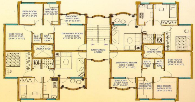
TYPICAL FIRST, SECOND AND THIRD FLOOR PLAN
