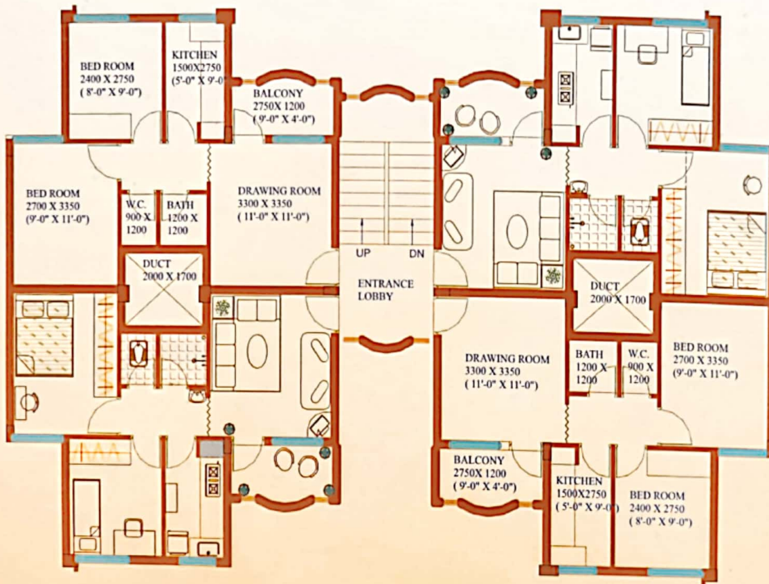
TYPICAL FIRST, SECOND AND THIRD FLOOR PLAN
