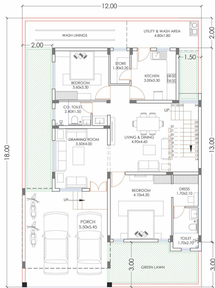
ENTRANCE GROUND FLOOR PLAN
