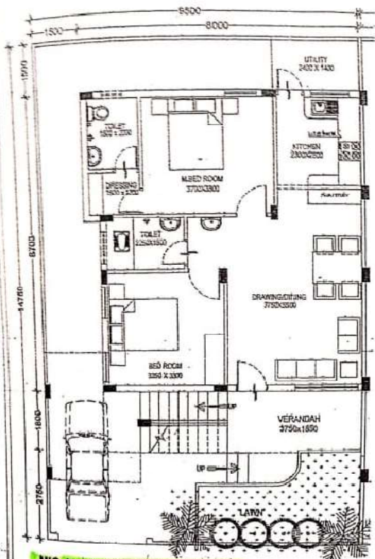
MIG Jr. - GROUND FLOOR PLAN
