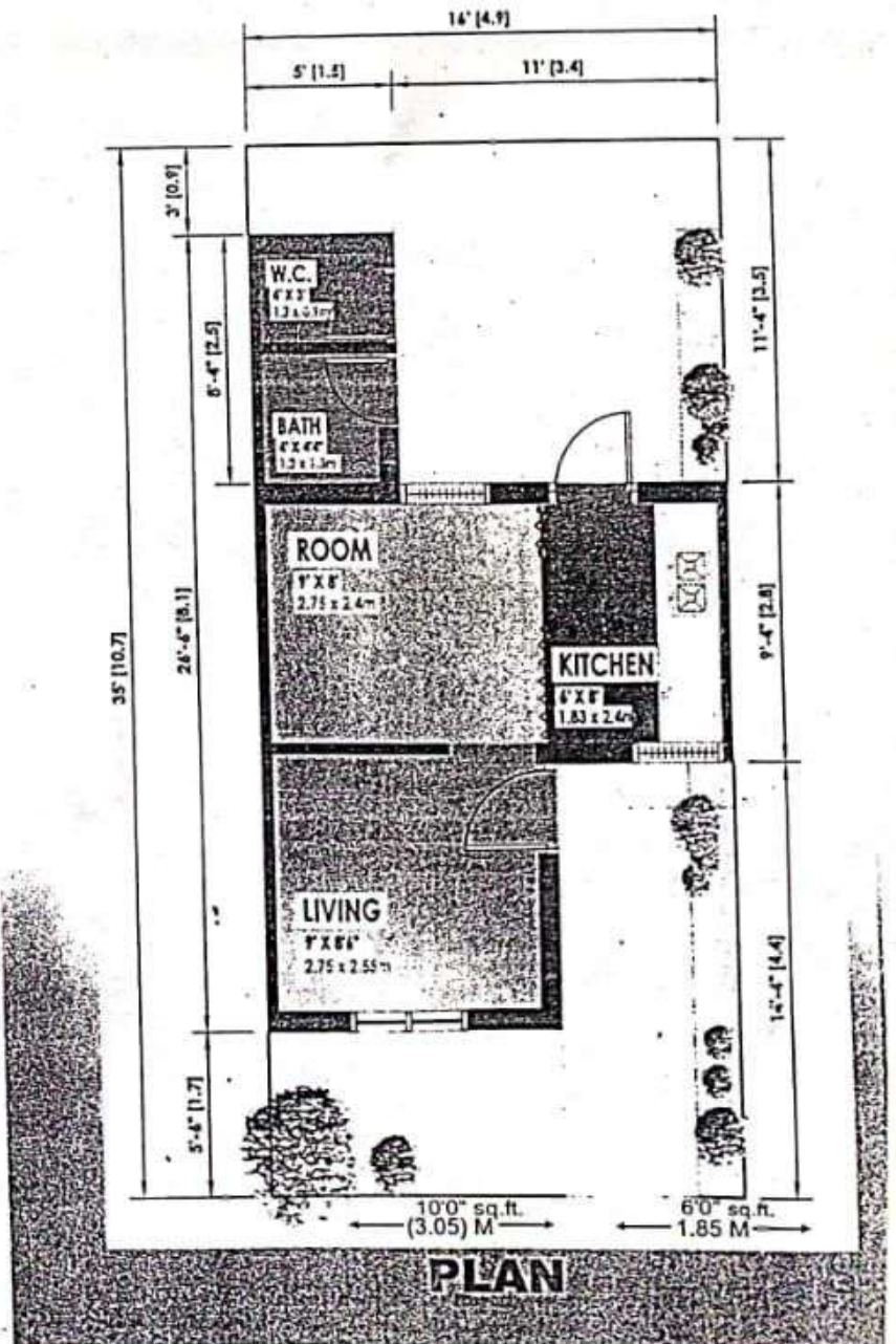
GROUND - FLOOR (भू - तल)
