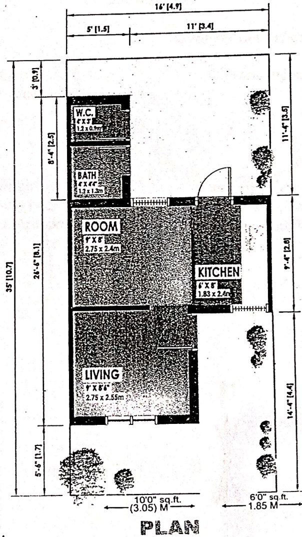
GROUND - FLOOR (भू - तल)
