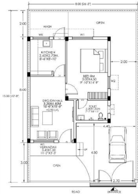
GROUND FLOOR PLAN [LIG-II]
