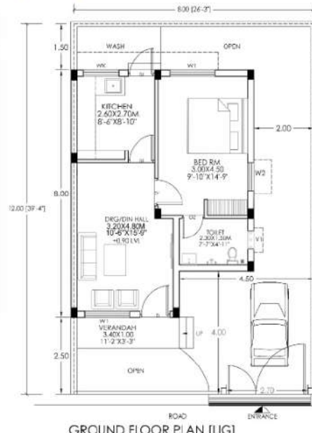
GROUND FLOOR PLAN [LIG]
