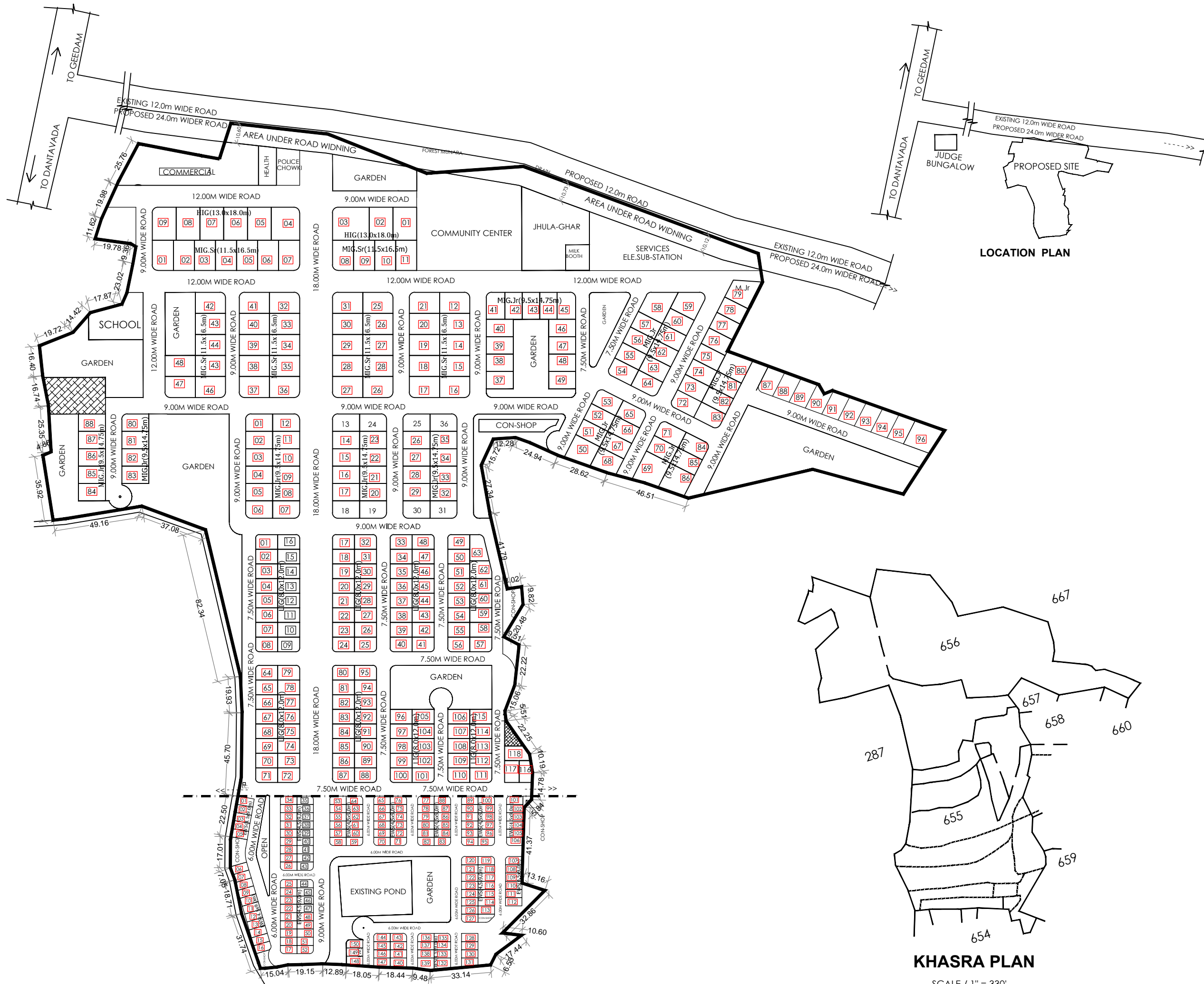
LAY OUT PLAN
